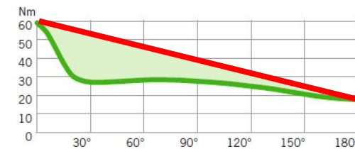
Reduction in opening effort thanks to EASY OPEN cam-action technology
